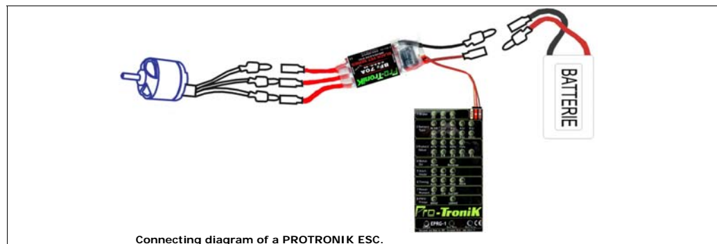
Connecting diagram of a PROTRONIK ESC.
